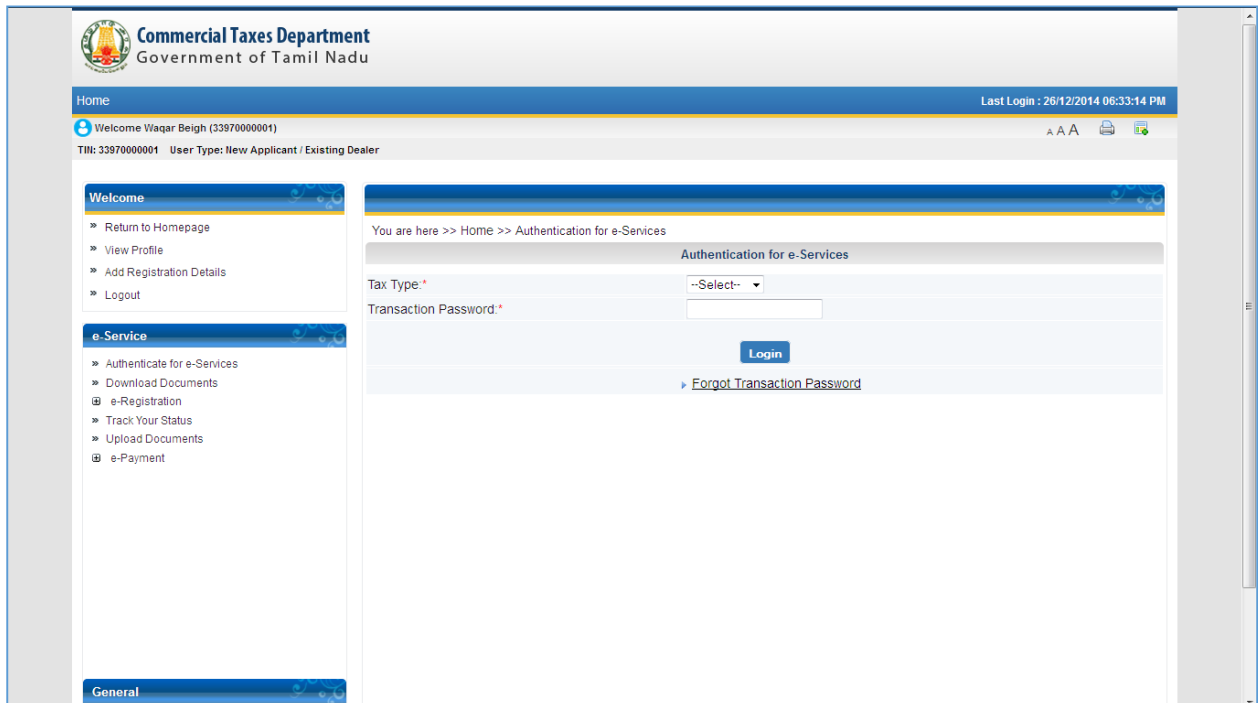
Figure 3: Authenticate Screen
