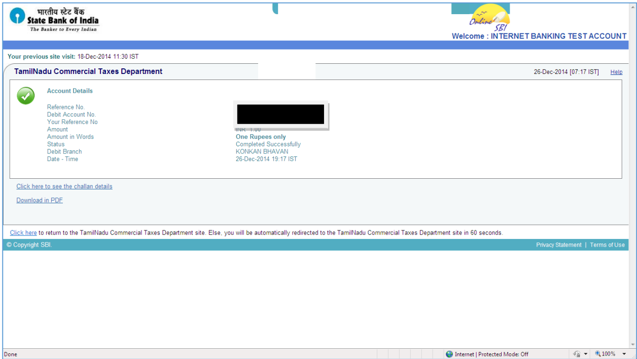
Figure 17: Payment Status
