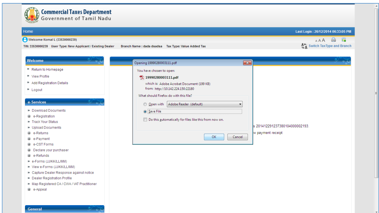
Figure 26: Download e-Challan
