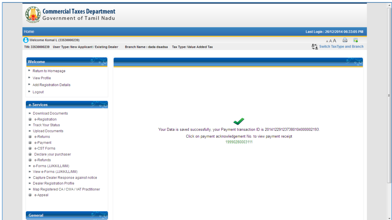
Figure 25: Challan Screen
