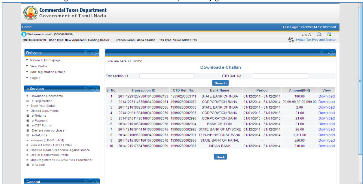
Figure 33: Download e-Challan
