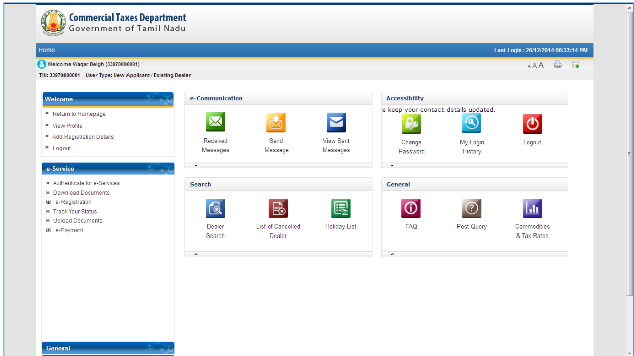
Figure 2: Home Screen
