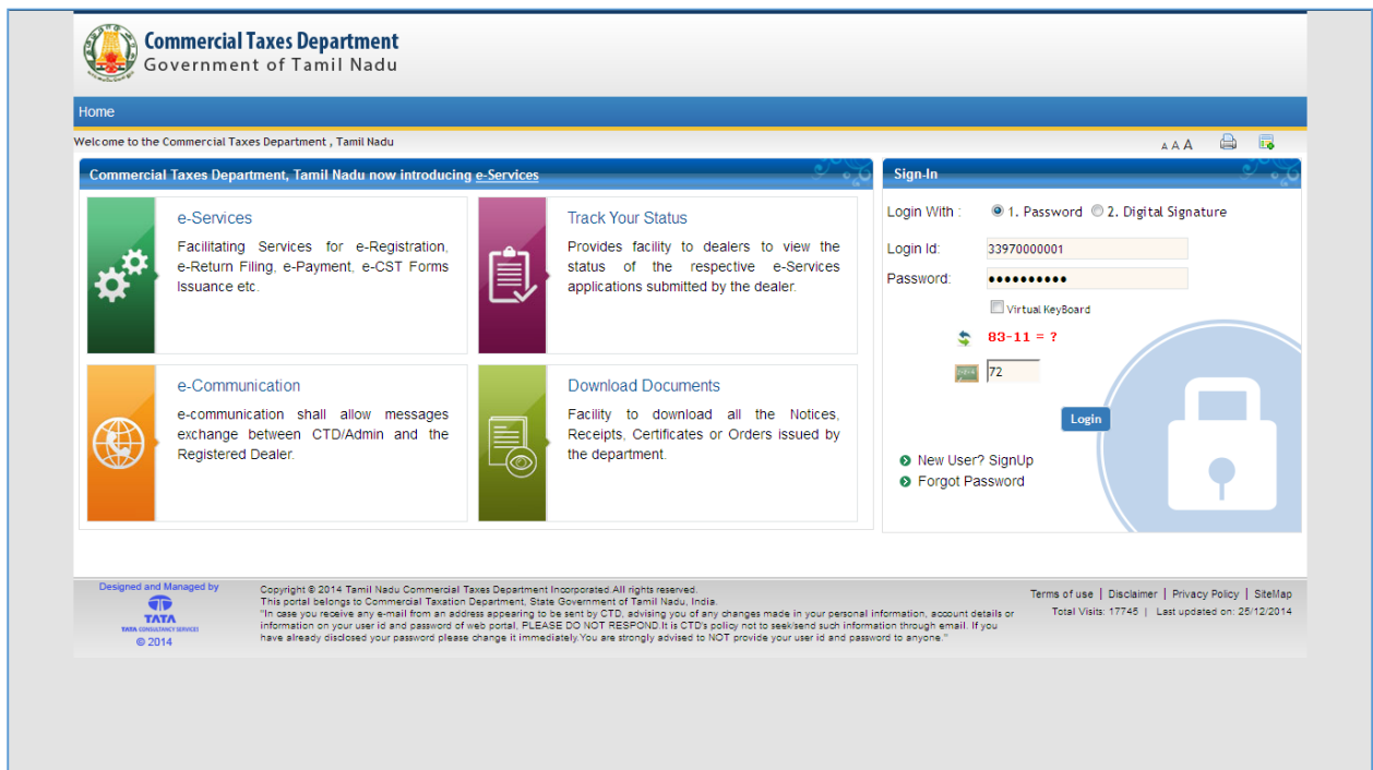
Figure 1: Login Screen
