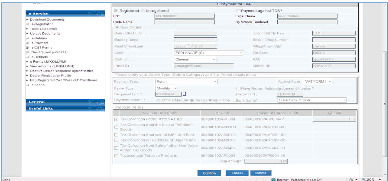
Figure 12: Confirm Payment
