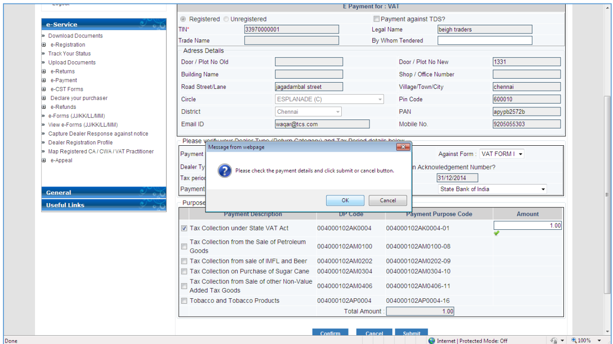
Figure 11: Confirm Payment
